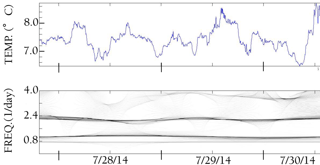
The oscillating temperatures recorded over a three-day period off Homewood is pictured above. Converting these oscillations using 'synchrosqueezing' is shown in the lower panel.
