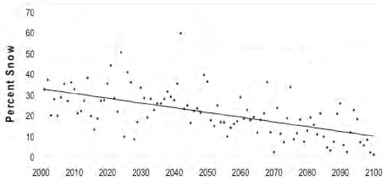
The decline in the percentage of precipitation as snow in the next 100 years under the GFDL-A2 scenario.
