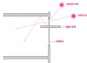
A light shelf that divides a window into a view section below and a clerestory section above.
