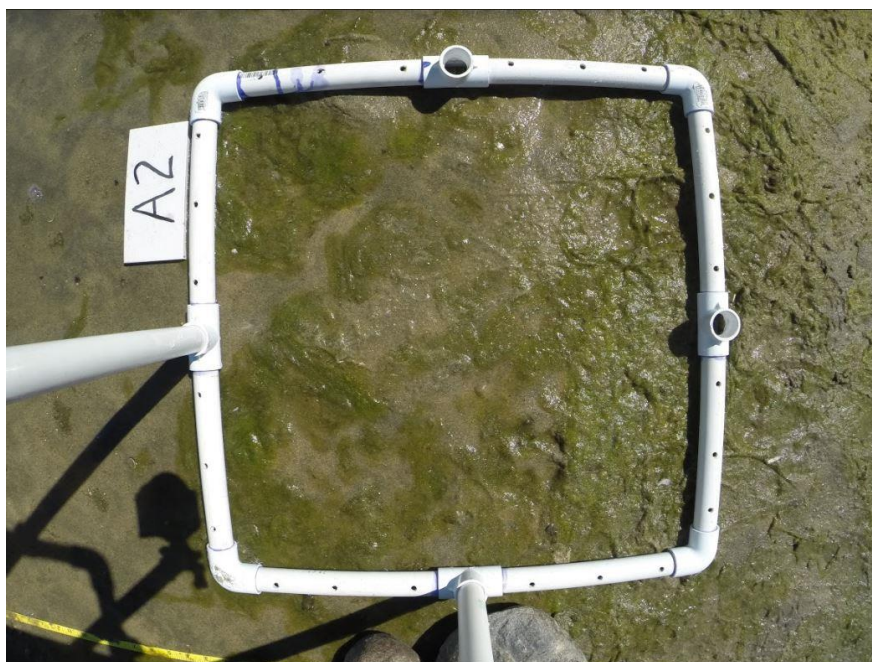
Figure 26 . Regan Beach 8/20/15 shoreline site A-2. The metaphyton algae was mostly various shades of green. The site had higher chlorophyll a relative to AFDW organic content (see Figure 24 above.)
